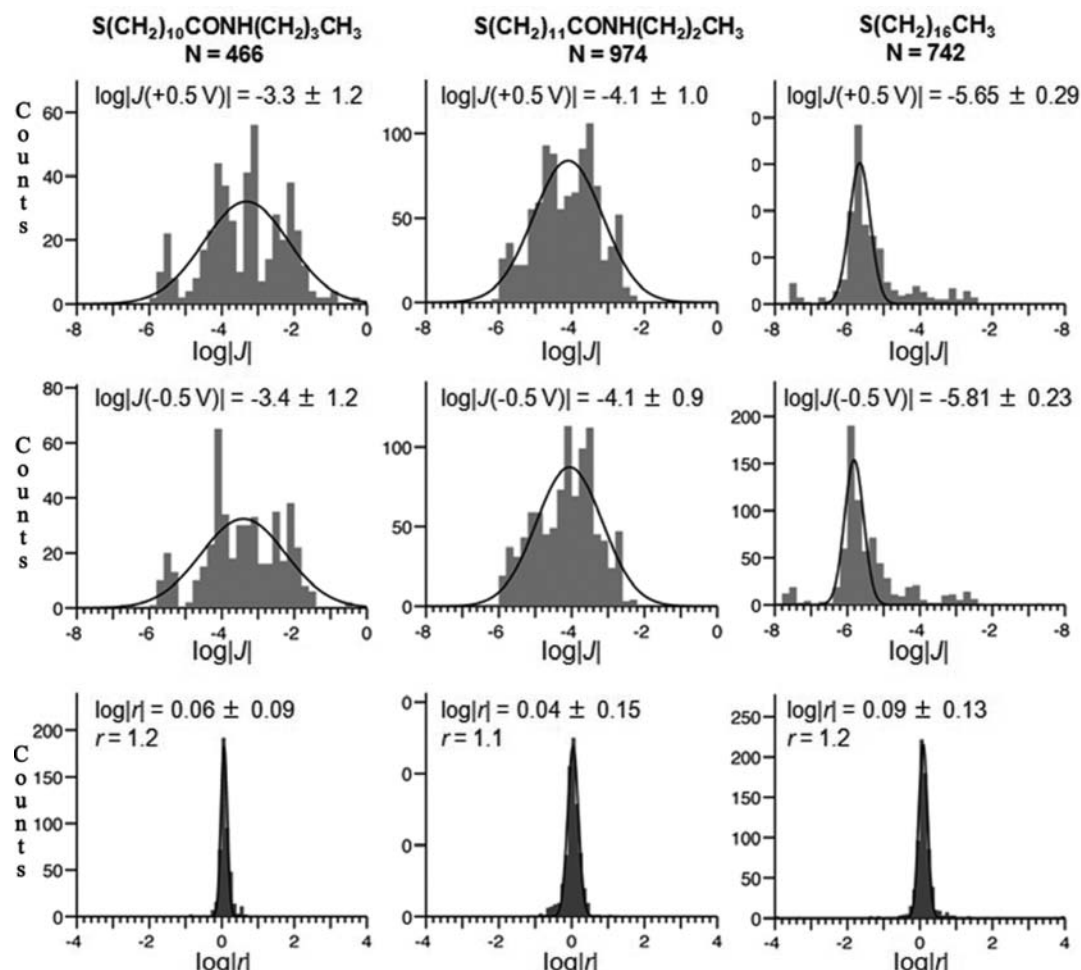
Figure 5. Histograms of \log|J| at opposite biases, +0.5 V (top row) and -0.5 V (middle row), above those of \log|r| (bottom row), where r = J(+0.5 V)/J(-0.5 V) , for two compounds with internal amides along the molecular backbone and an n -alkanethiol. The first two rows of histograms illustrate the effect of reversing the applied bias on the distribution of the histograms. The bottom row of histograms gives the histogram of rectification ratios for the three molecules. Comparison down each column illustrates the difference between the width of distributions for current density at opposite applied biases and the rectification ratios.
