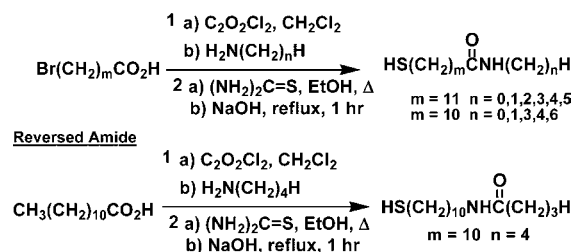
Scheme 1. Synthesis of Mercapto- N -alkylamides ( m = 10 or 11 ) from the Respective Primary Bromocarboxylic Acid via a Bromoalkylamide a
